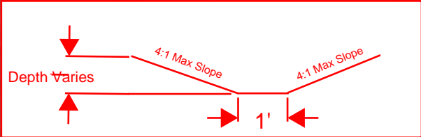
Section A-A Drainage Swale -NTS-
