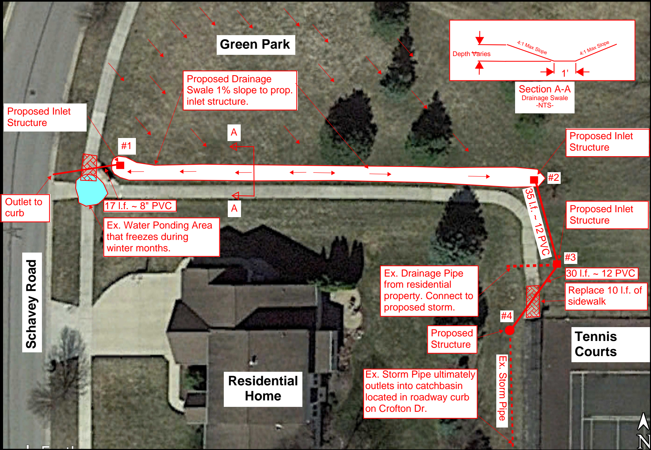
Option #4 Split Drainage to Tennis Courts
